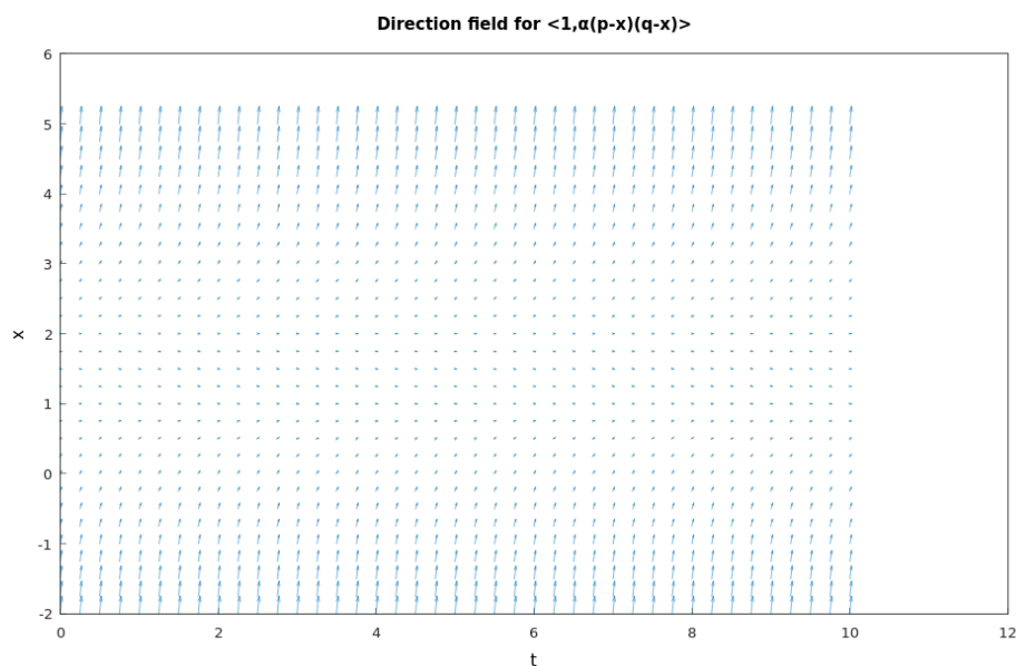
Figure 5.57: The direction field for \langle 1, \alpha(p - x)(q - x) \rangle with \alpha = 1 , p = 1 , and q = 2 (Hamzstplot/Examples with Makefile/Differential Equations/Plot Direction Fields for Chemical Reactions Problem 28a/main.cpp).
