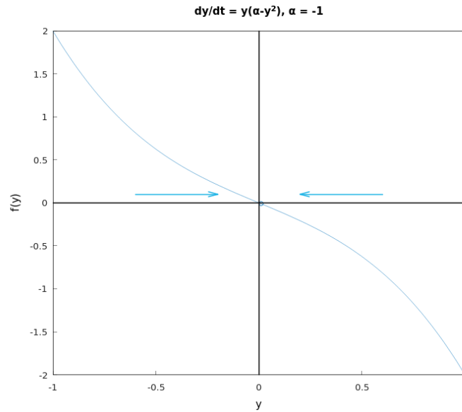
Figure 5.50: The plot for f(y) = y(\alpha - y^2) with \alpha = -1 , the phase line is drawn with the blue arrows ( Hamzstplot/Examples with Makefile/Differential Equations/Plot 2D for Bifurcation Points Problem 26 Only 1 Equilibrium Solution/main.cpp ).
