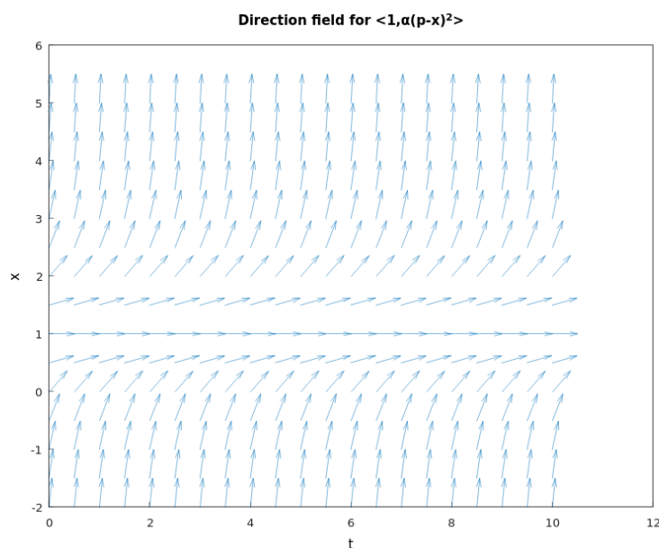
Figure 5.58: The direction field for \langle 1, \alpha(p-x)^2 \rangle with \alpha = 1 and p = 1 (Hamzstplot/Examples with Make-file/Differential Equations/Plot Direction Fields for Chemical Reactions Problem 28b/main.cpp).
