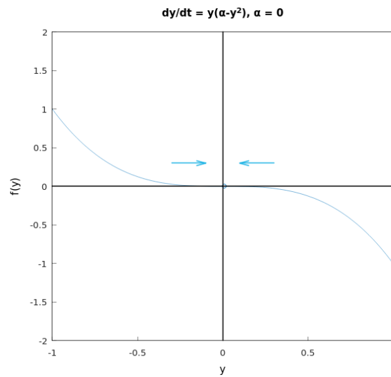
Figure 5.51: The plot for f(y) = y(\alpha - y^2) with \alpha = 0 , the phase line is drawn with the blue arrows ( Hamzstplot/Examples with Makefile/Differential Equations/Plot 2D for Bifurcation Points Problem 26 Only 1 Equilibrium Solution/main.cpp ).
