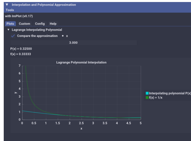
Figure 11.7: The plot for Lagrange interpolating polynomial with Hamzstlab, SymIntegration and Armadillo for f(x) = \frac{1}{x} with nodes x_0 = 2, x_1 = 2.5 , and x_2 = 4 . (Hamzstlab-Mathematics/examples/Interpolation/main.cpp).
