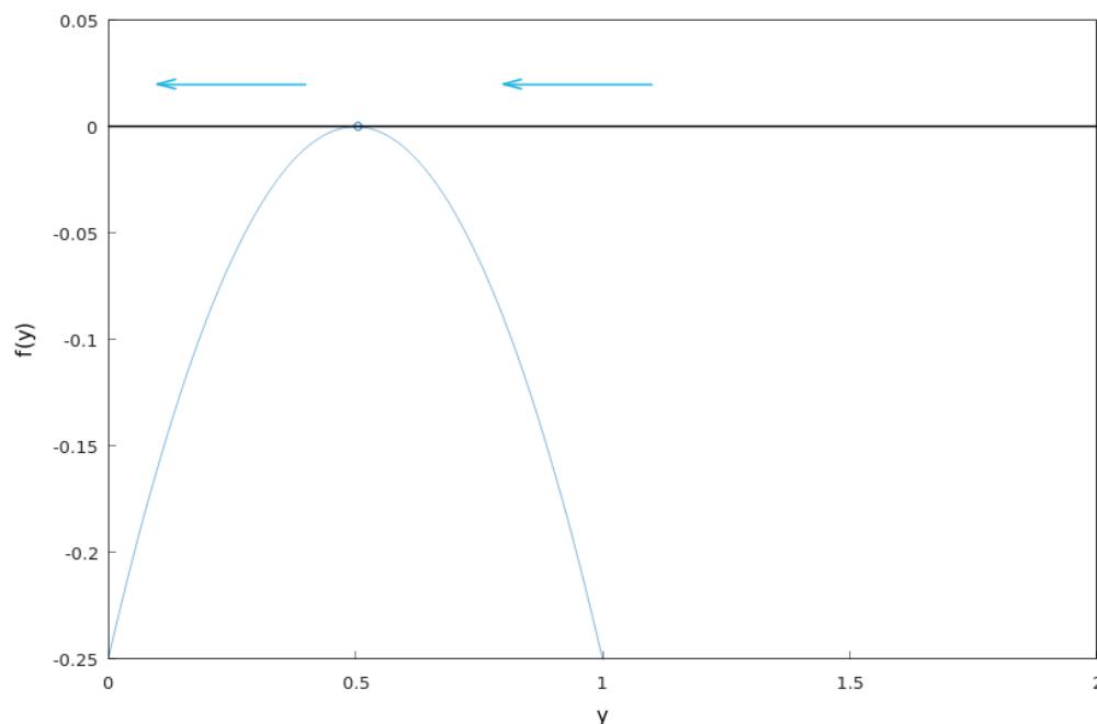
Figure 5.41: The plot for f(y) = (1-y)y - \frac{1}{4} (Hamzstplot/Examples with Makefile/Differential Equations/Plot 2D Equilibrium Solution Only 1 for Schaefer Model Variation/main.cpp).
