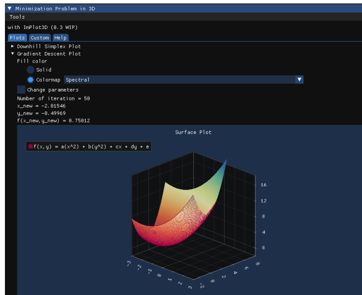
Figure 11.13: The interactive surface plot for f(x, y) = \frac{1}{2}x^2 + 2x + y^2 + y + 3 with Hamzstlab Mathematics and SymIntegration combined so you can see the optimum / minimum value there. (Hamzstlab-Mathematics/examples/3D Minimization/main.cpp).
