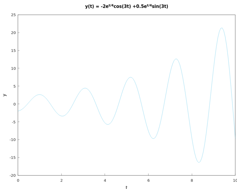
Figure 5.72: The graph of the solution y = -2e^{t/4} \cos 3t + \frac{1}{2}e^{t/4} \sin 3t of the initial value problem 16y'' - 8y' + 145y = 0, y(0) = -2, y'(0) = 1 (Hamzstplot/Examples with Makefile/Differential Equations/Plot 2D Growing Oscillation/main.cpp).
